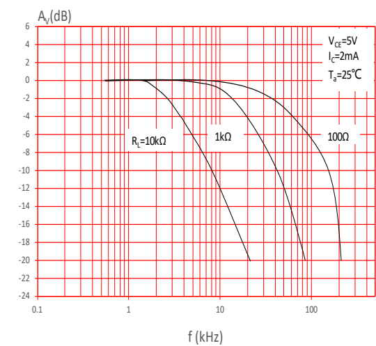
FIG.10: Frequency Response
