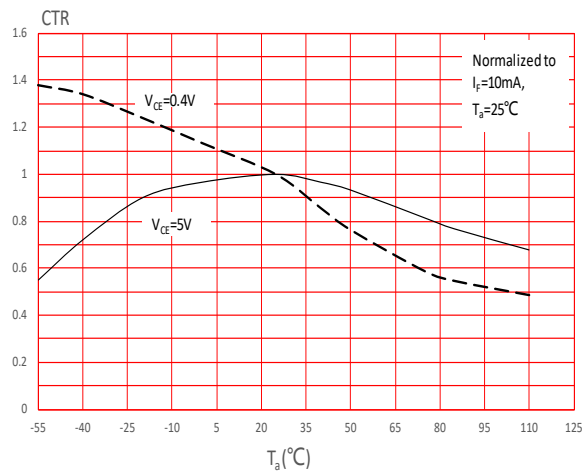
FIG.7: Normalized Current Transfer Ratio vs. Ambient Temperature
