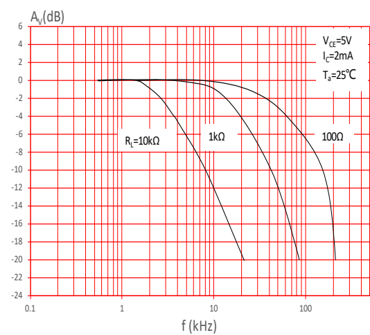
FIG.10: Frequency Response
